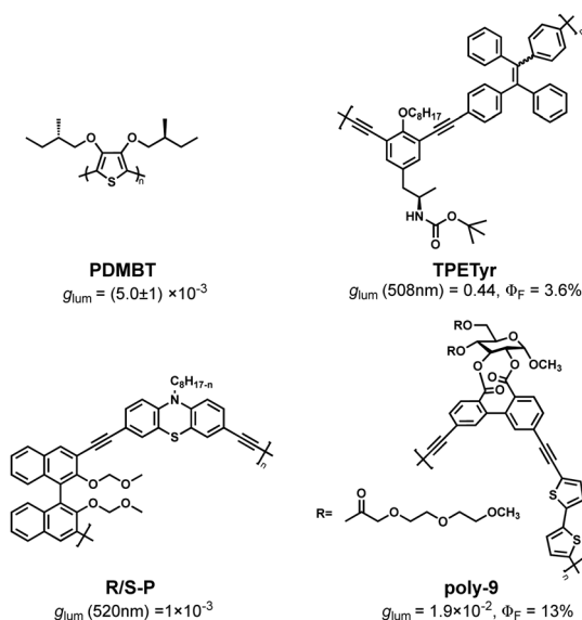
Fig. 1 Chemical structures of optically active helical polymers.
