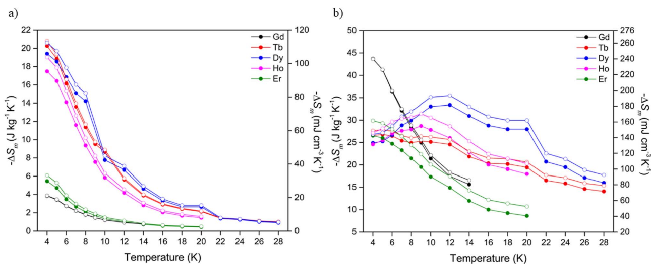
Fig. 3 Magnetic entropy changes of the \text{Ln}(\text{OH})_3 series for (a) \Delta B = 1\text{-}0 \text{ T} and (b) \Delta B = 5\text{-}0 \text{ T} . The filled and open symbols denote mass and volumetric entropy units respectively.
