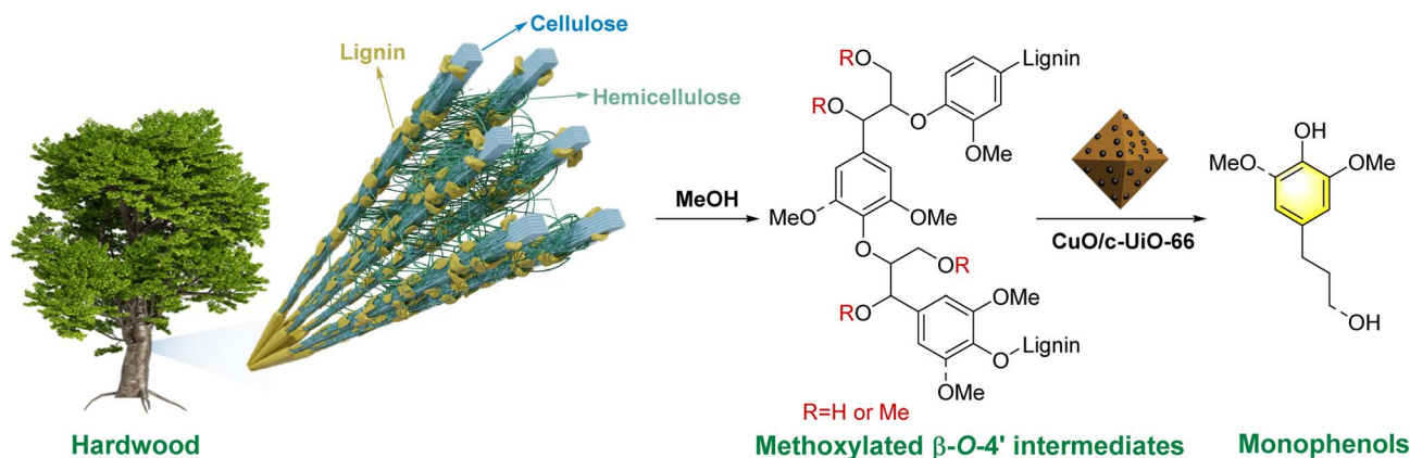
Fig. 7 Plausible reaction pathway for the reductive catalytic decomposition of lignin from woody biomass into phenolic monomers over the CuO/c-UiO-66 catalyst.
