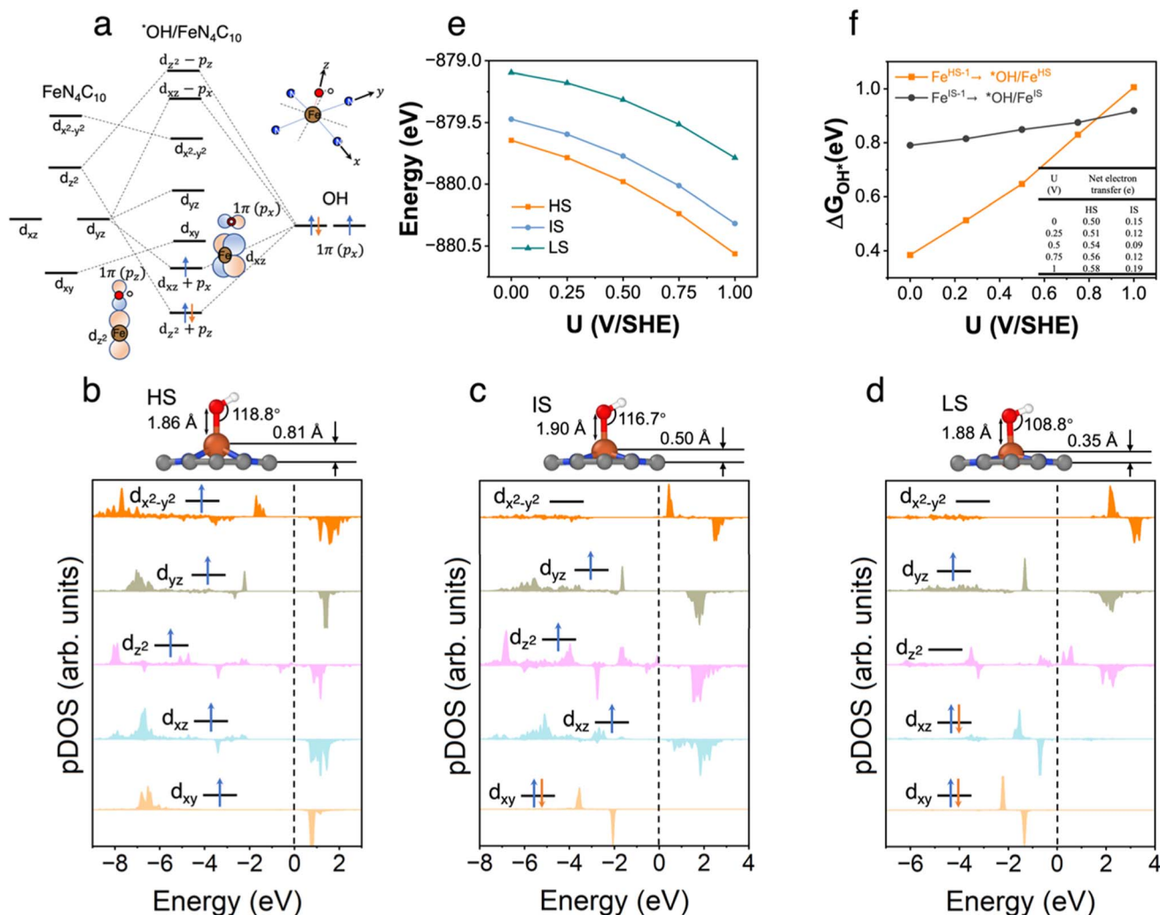
Fig. 5 *OH/FeN_4C_{10} . (a) Schematics of orbital hybridizations of Fe 3d orbitals in a square-planar ligand field with the 2p orbitals in the OH adsorbate. (b)–(d) Atomic structures and pDOS plots of the HS, IS, and LS states of *OH/FeN_4C_{10} . (e) Spin- and potential-dependent energies of *OH/FeN_4C_{10} under constant-potential conditions. (f) Spin and potential-dependent *OH adsorption energies. The inset table shows the net electron transfer in the adsorption process.
