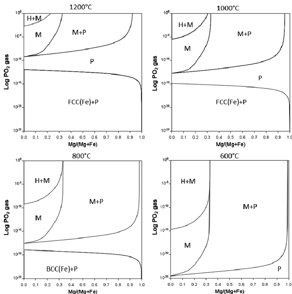
Fig. 13 Mg/(Mg + Fe) vs. activity of \log P_{O_2} in gas at 1200, 1000, 800 and 600 °C where M = magnetite ( Fe,Mg_3O_4 ), H = hematite ( Fe_2O_3 ), P = periclase ( Fe,MgO ) calculated using Thermo-Calc software TCOX Metal Slag and Oxides Database version 11.
