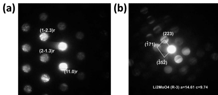
Fig. 2 Examples of electron diffractions taken from Mo-doped NC90 material. (a) CBED pattern indexed in terms of \text{Li(TM)}\text{O}_2 phase. Label “r” denotes a rhombohedral ( R\bar{3}m ) structure. (b) CBED pattern associated with the \text{Li}_2\text{MoO}_4 phase.
