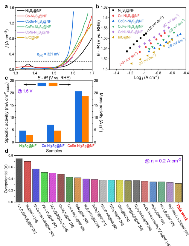
Fig. 4 Electrochemical properties of catalysts for OER. (a) OER polarization curves and (b) Tafel plots of \text{Ni}_3\text{S}_2\text{@NF} and \text{CoSn-Ni}_3\text{S}_2\text{@NF} with Ir/C@NF. (c) Specific activities and mass activities of \text{Ni}_3\text{S}_2\text{@NF} , \text{Co-Ni}_3\text{S}_2\text{@NF} , and \text{CoSn-Ni}_3\text{S}_2\text{@NF} . (d) Comparison of \eta at 0.2 \text{ A cm}^{-2} for \text{CoSn-Ni}_3\text{S}_2\text{@NF} with previously reported results for other nickel-based catalysts.
