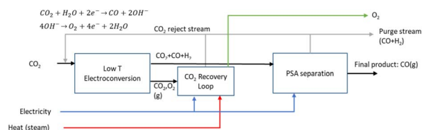
Fig. 4 Process diagram of the LT CO 2 electrolysis towards CO.
