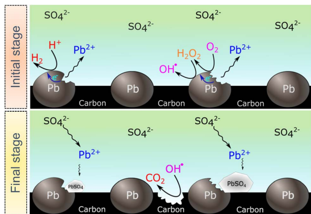
Fig. 4 Proposed mechanism for carbon additive degradation and accelerated sulfation in the presence of ROS. Showing the HER and ORR taking places on the Pb particles at the initial stage, followed by the sulfation process and carbon binder degradation by the \text{OH}^{\bullet} forming \text{CO}_2 .
