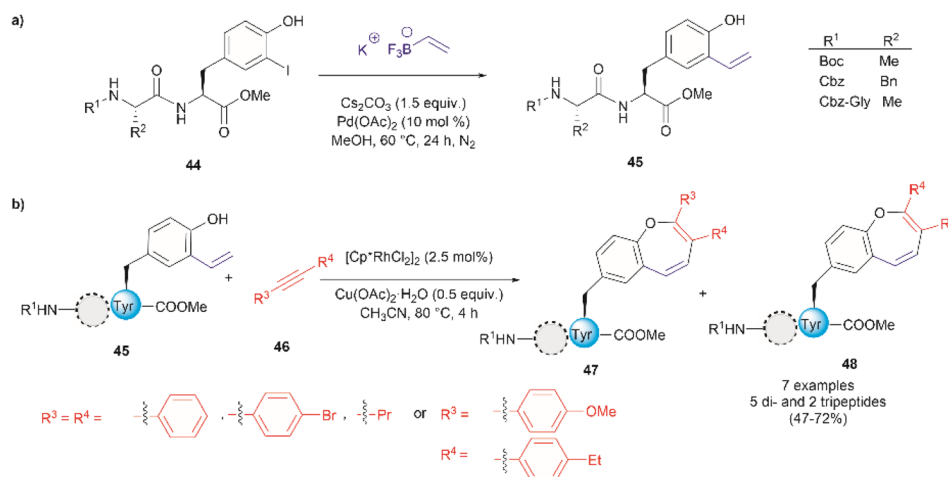
Fig. 12 (a) Suzuki–Miyaura cross coupling reaction for the preparation of ortho -vinylylated Tyr peptides. (b) Rh-catalyzed annulation of ortho -vinylylated Tyr with alkynes to give functionalized oxepine peptides.
