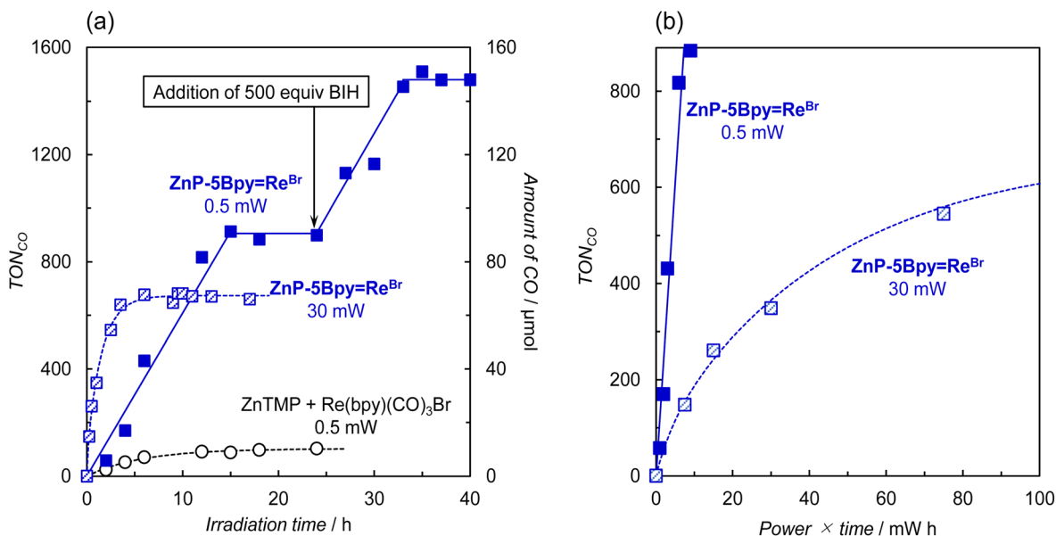
Fig. 10 (a) Time dependence of CO formation during irradiation at 420 nm by LED lamps (input power: 0.5 and 30 mW), in a merry-go-round irradiation apparatus, of CO 2 -saturated DMA-TEOA (4 : 1 v/v) solutions containing ZnP-5Bpy=Re Br (0.05 mM), and a mixed system of ZnTMP (0.05 mM) and fac -Re(bpy)(CO) 3 Br (0.05 mM) in the presence of BIH (0.05 M). (b) Plots of TON CO versus product of input power and irradiation time.
