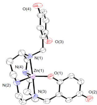
Fig. 1 ORTEP representation of the structure of [\text{Zn}^{\text{II}}(\text{H}_3\text{qp4})]^+ . The triflate counteranion and all H atoms are omitted for clarity. All ellipsoids are drawn at 50% probability. Full crystallographic data are provided in the ESI and in the Cambridge Structural Database (number 2173563†).
