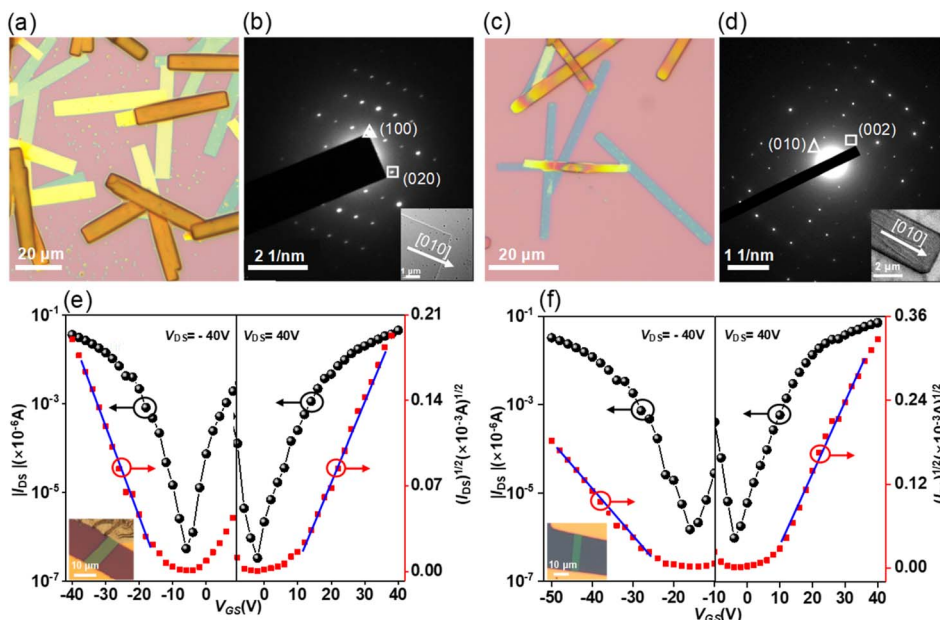
Fig. 8 Optical microscopy images of microbelts 9 (a) and 9 · C 60 (c); the selected-area electron diffraction (SAED) patterns of microbelts 9 (b) and 9 · C 60 (d) (inset: the TEM image of a single-crystalline microbelt); the transfer characteristics of an OFET based on microbelts 9 ( W/L = 7.8/22.1 ) (e) and 9 · C 60 ( W/L = 4.8/23.3 ) (f).
