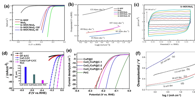
Fig. 7 (a) Linear sweep voltammograms of Er-MOF/MoS 2 , MoS 2 , and Er-MOF, in 0.5 M H 2 SO 4 at a scan rate of 5 mV s -1 . (b) The corresponding Tafel plots of Er-MOF/MoS 2 , MoS 2 . (c) Cyclic voltammetry of Er-MOF/MoS 2 in the non-Faraday potential region at different scanning rates in 0.5 M H 2 SO 4 . Copyright 2022, Elsevier. (d) Polarization curves of carbon cloth (CC), ZIF-8/CC, CoP-C/CC, CeO 2 -CoP-C/CC, and Pt/C in a N 2 -saturated 0.5 M H 2 SO 4 solution. Scan rate: 2 mV s -1 . Inset shows the corresponding overpotential of CoP-C/CC, CeO 2 -CoP-C/CC, and Pt/C at the current density of 10 mA cm -2 ( \eta_{10} ). Copyright 2018, Elsevier. (e) Polarization curves of HER, Copyright 2021, Wiley VCH. (f) The corresponding Tafel plots for HER, Copyright 2021, Wiley VCH.
