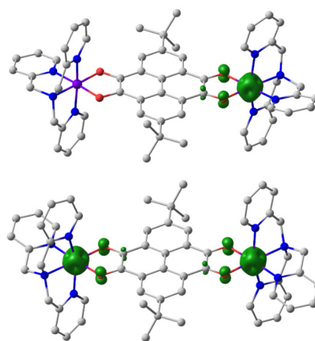
Fig. 9 Spatial structure and spin density distribution (contour value = 0.03 \text{e}^{-3} ) of compound 3 in the \{\text{Co}^{\text{III-LS}}(\text{tpa})\text{-pyrene}^{\text{Cat-Sq-CO}^{\text{II-HS}}(\text{tpa})}\} (top) and \{\text{Co}^{\text{II-HS}}(\text{tpa})\text{-pyrene}^{\text{Sq-Sq-CO}^{\text{II-HS}}(\text{tpa})}\} (bottom) charge distributions, as calculated by the DFT UTPSSH/6-311++G(d,p) method. Hydrogen atoms and counter-ions are omitted for clarity.
