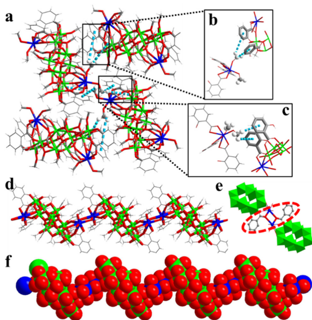
Fig. 2 In (\text{Ti}_{10}\text{Cu}_2)_{\text{sp}} , the \text{CH}\cdots\pi interactions of inter-clusters between \text{Sal}^{2-} ligands and -\text{OMe} (a). (b and c) Enlarged view of the area outlined in (a). In (\text{Ti}_{10}\text{Cu}_2)_{\text{cs}} , view of the chain structure (d), "Sal-Cu" units (e) and space-filling view of the chain (f). Colour code and representation: Ti, green; Cu, blue; O, red; C, grey; H, white; \text{CH}\cdots\pi interactions, dashed cyan lines.
