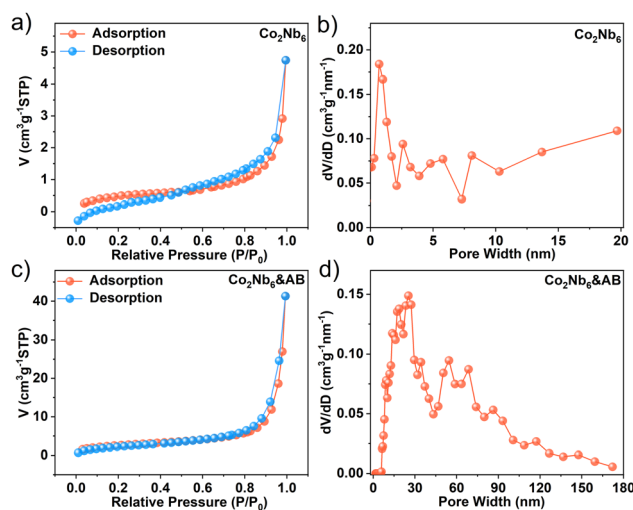
Fig. 4 N 2 adsorption–desorption isotherms of (a) \text{Co}_2\text{Nb}_6 and (c) \text{Co}_2\text{Nb}_6\&\text{AB} ; and pore size distribution curves for (b) \text{Co}_2\text{Nb}_6 and (d) \text{Co}_2\text{Nb}_6\&\text{AB} .
