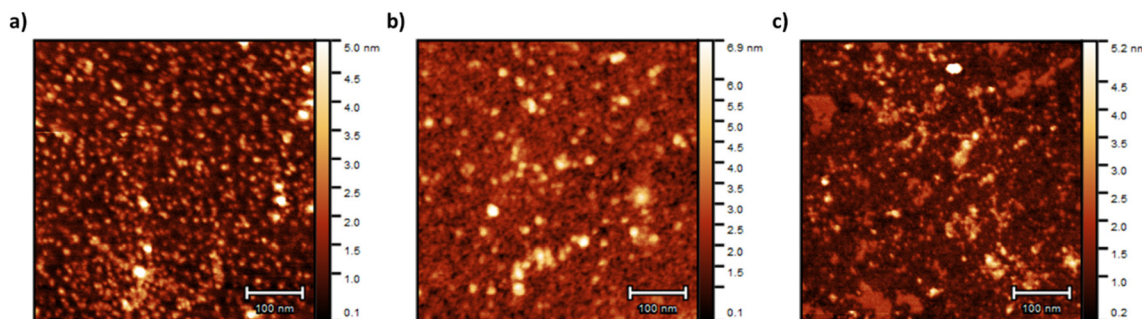
Fig. 4 AFM pictures of (a) Star 1, (b) Star 2 and (c) Star 3. The samples were prepared at 0.025 \text{ mg mL}^{-1} onto freshly cleaved mica.
