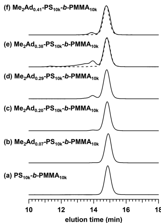
Fig. 5 SEC traces of Me 2 Ad-PS 10k - b -PMMA 10k samples (b)–(f) and the corresponding PS 10k - b -PMMA 10k (a) (eluent, THF; flow rate, 1.0 mL min -1 ). The dashed curves represent the SEC traces after preparative SEC purification.
