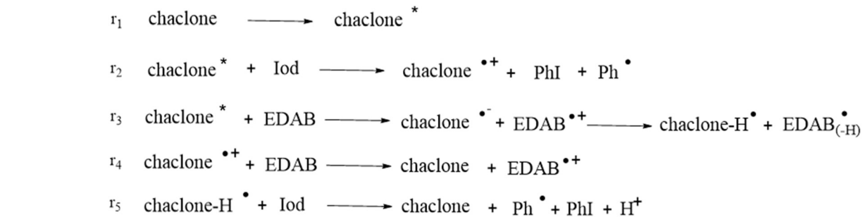
Fig. 8 Proposed photopolymerization mechanisms for TPA-2 and the chalcones.
