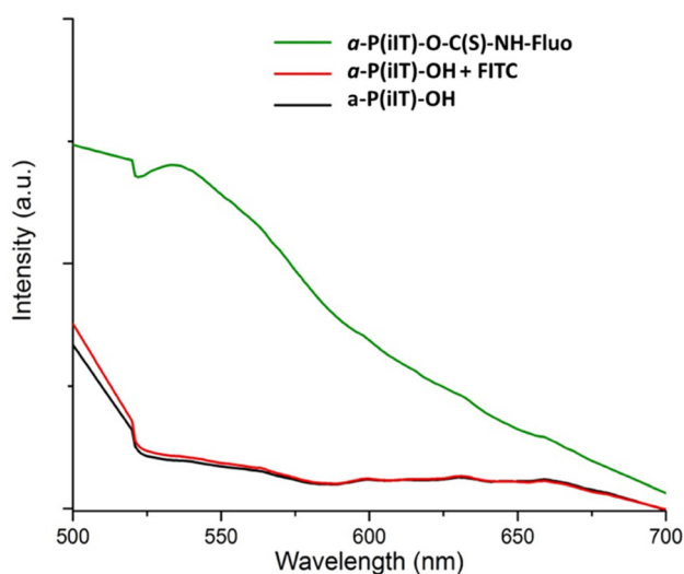
Fig. 6 Fluorescence emission studies for a -P(iIT)-OH (control, black line), a -P(iIT)-OH dipped in fluorescein solution (control, red line) and fluorescein-functionalized a -P(iIT)-O-C(S)-NH-Fluo (green line) thin films on SiO 2 in the solid state. All samples were excited at 495 nm and monitored for fluorescence emission between 500–700 nm.
