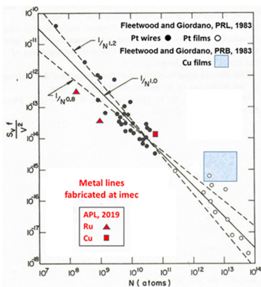
Fig. 9 S_v f/V^2 at 295 K and f = 10 Hz for Pt NWs fabricated by substrate step lithography (solid black circles); mechanically scribed, sputtered Pt films (open circles); and mechanically scribed, thermally evaporated Cu films (large, blue box). Lines are proportional to 1/N^{\alpha} ( \alpha = 1.0 \pm 0.2 ). Results are compared with Ru (length L = 10 \mu\text{m} and 50 \mu\text{m} ) and Cu resistors fabricated at imec (small red box). Adapted from ref. 71 with permission. Copyright 2019 American Institute of Physics.
