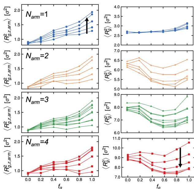
Fig. 5 Dependence of the mean-squared radius of gyration of arms (left panels) and stars (right panels) to degree-of-protonation, f_q at different values of N_{arm} . Arrow denotes increasing f_q . Connecting lines are data points with the same \phi_s .
