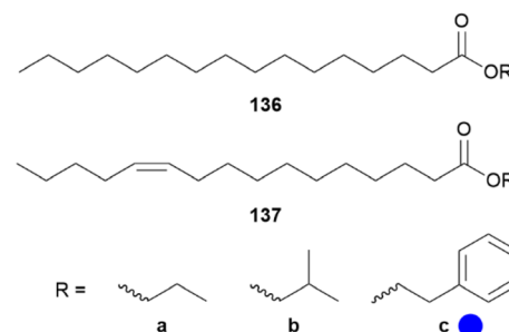
Fig. 28 Wing-specific ester of androconia of Bicyclus martius sanaos . The colour code indicates occurrence only in a single family (•).
