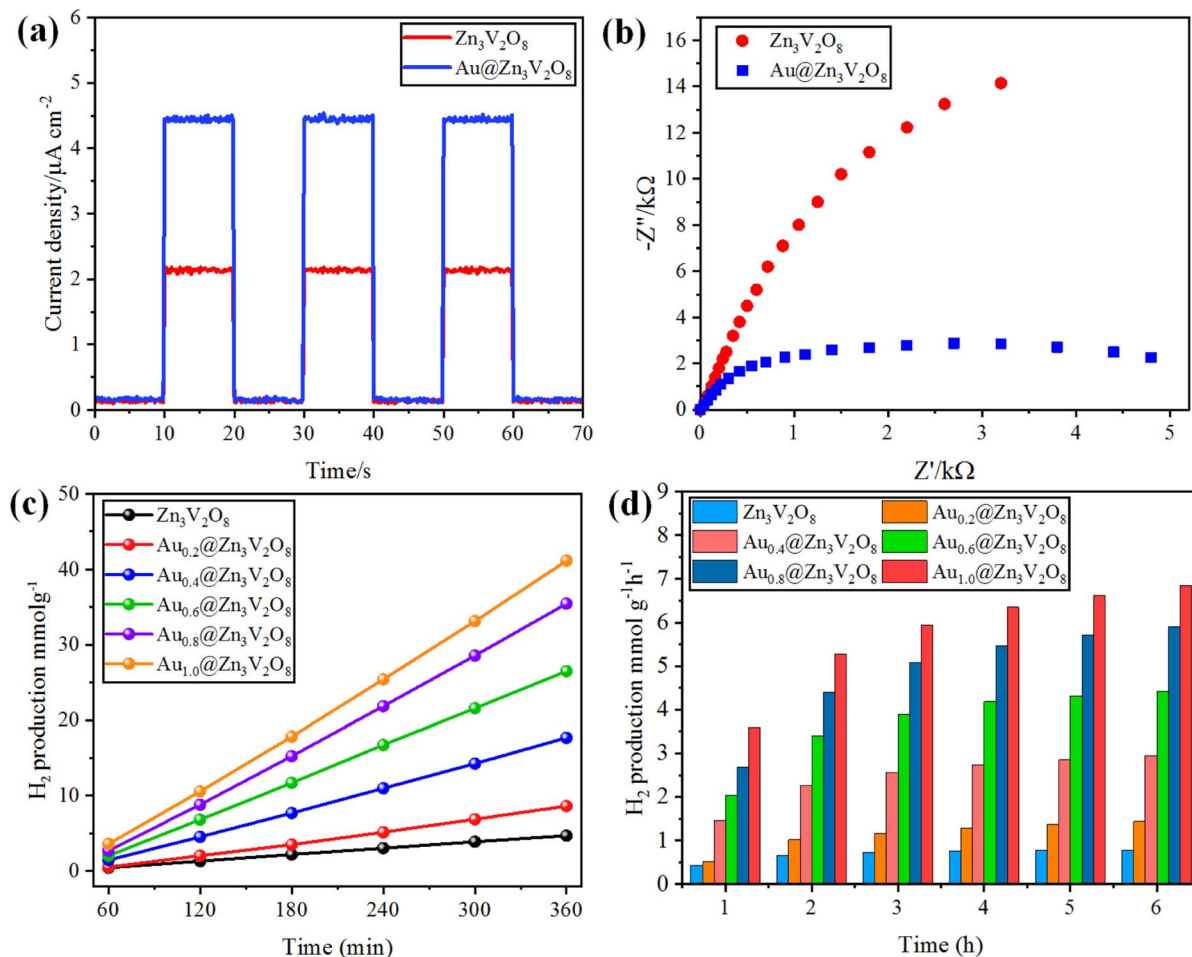
Fig. 7 (a) Photocurrent response, (b) EIS results of Zn 3 V 2 O 8 and Au@Zn 3 V 2 O 8 . (c and d) comparison of the photocatalytic activities of the photocatalysts in mmol g -1 and mmol g -1 h -1 , respectively.
