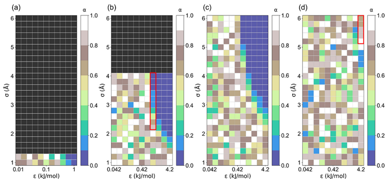
Fig. 6 The correlation between step location ( \alpha ) and LJ parameter ( \sigma and \varepsilon ) for (a) l = 5 , (b) l = 7.5 , (c) l = 10 and (d) l = 35 Å structures.
