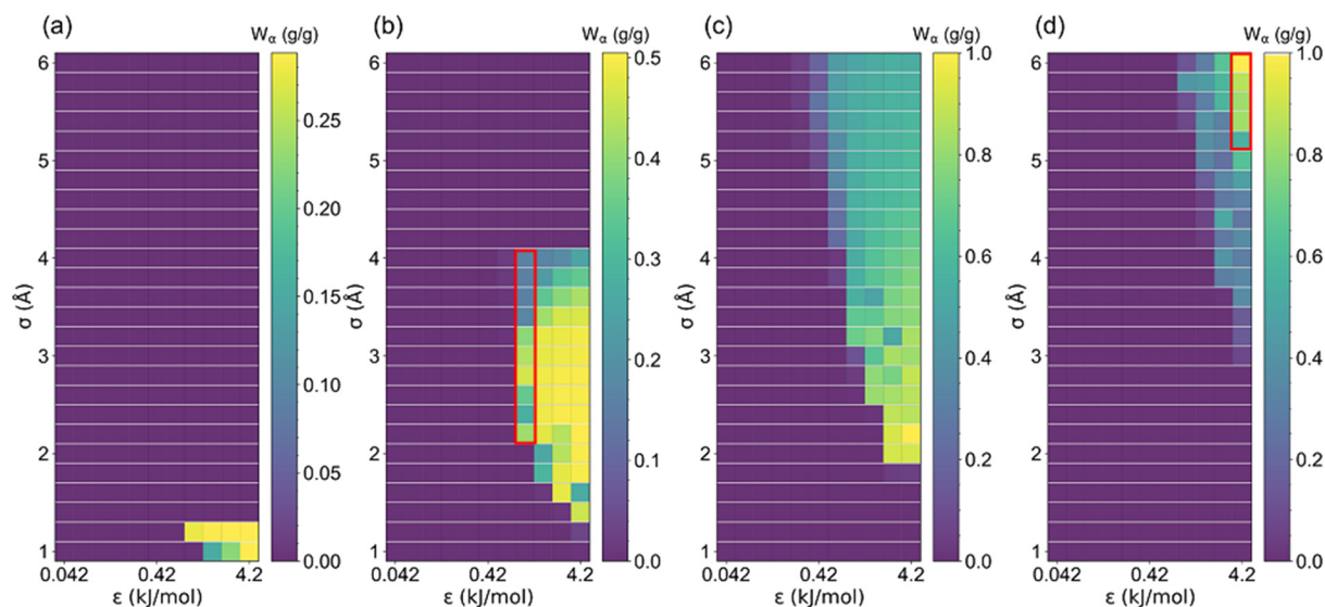
Fig. 7 The uptake change at step location ( W_\alpha ) changed with LJ parameter ( \sigma and \varepsilon ) for (a) l = 5 , (b) l = 7.5 , (c) l = 10 and (d) l = 35 Å structures.
