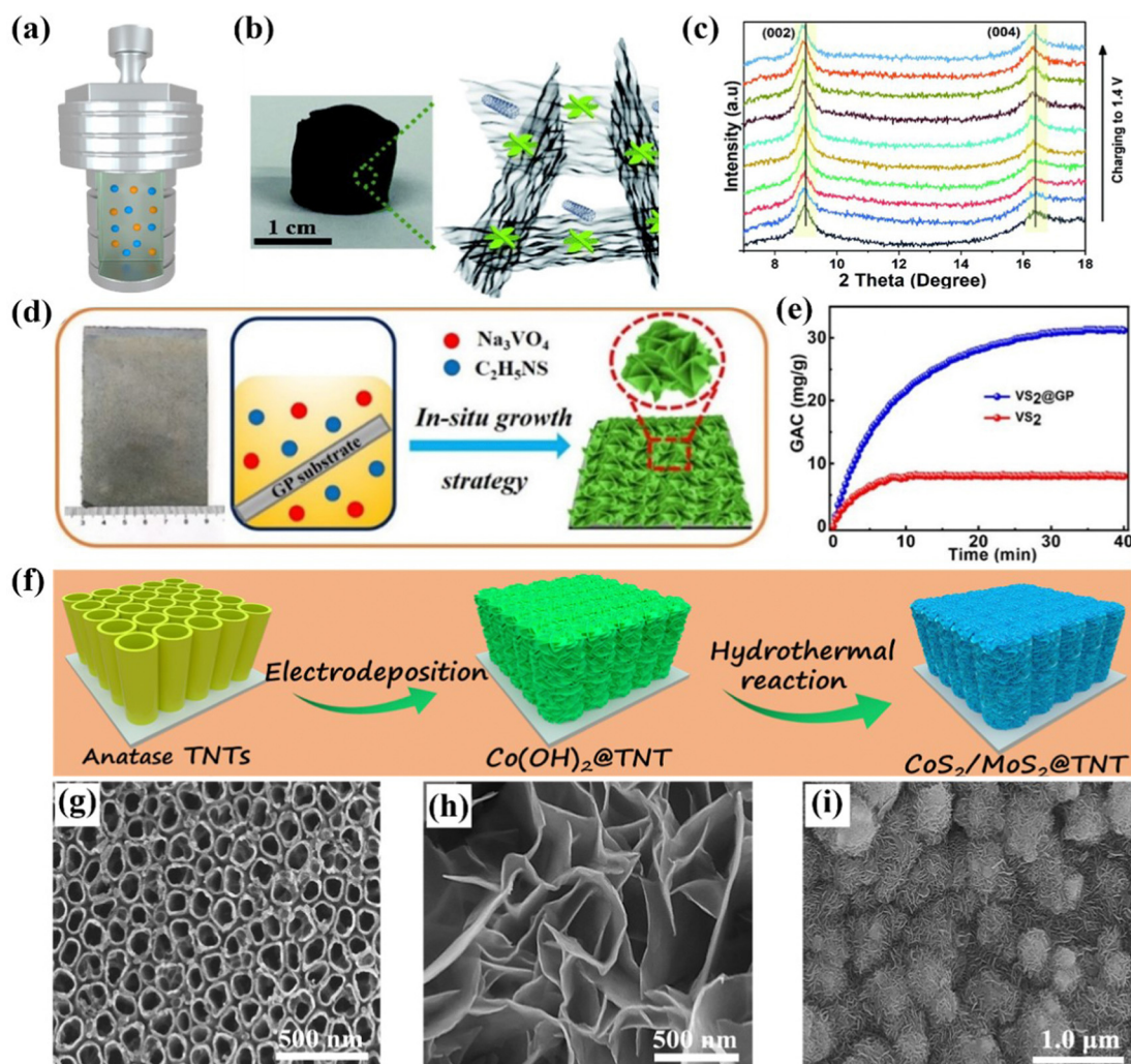
Fig. 6 (a) Schematic illustration of hydrothermal/solvothermal methods. (b) Photograph and schematic and (c) in situ XRD patterns during the charging step of \text{VS}_2/\text{rGO}-\text{CNT} aerogel, reproduced from ref. 131 with permission from the Royal Society of Chemistry. Schematic diagram of (d) preparation and (e) ion removal capacity of the self-supported \text{VS}_2@\text{GP} electrode, reproduced from ref. 132 with permission from the American Chemical Society. Schematic illustration of (f) the fabrication of \text{MoS}_2/\text{CoS}_2@\text{TiO}_2 nanotube hybrid electrodes, and SEM images of (h) \text{TiO}_2 nanotubes, (i) \text{Co}(\text{OH})_2 skeleton, and (j) hybrid electrode, reproduced from ref. 124 with permission from Elsevier.
