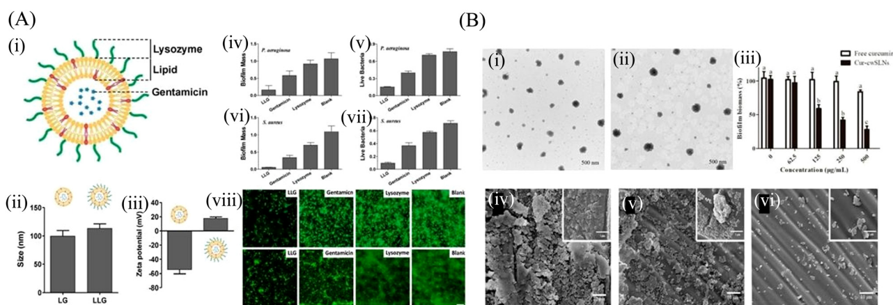
Fig. 5 (A) (i) Schematic structure of lysozyme-associated liposomal gentamicin (LLG), (ii) hydrodynamic size, and (iii) surface zeta potential of liposome (without Lysozyme) and LLG, Crystal violet assay and 3-(4,5-dimethyl-thiazol-2-yl)-2,5-diphenyltetrazolium bromide (MTT) assay to assess the antibiofilm activity of LLG against P. aeruginosa biofilm (iv and v) and S. aureus (vi and vii). Fluorescence microscopy of P. aeruginosa (viii) and S. aureus (ix) biofilms. Biofilms incubated with tryptic soy broth (TSB) are used as the control. Scale bars were 10 \mu\text{m} . (B) The TEM of the SLNs (i) cwSLN, (ii) Cur-cwSLN, (iii) the cytotoxicity of cwSLNs and Cur-cwSLNs in 24 h. Data are presented as the mean \pm SD, n = 3 , (iv) SEM image of S. aureus biofilms, (v and vi) SEM image of inhibitory effects of pure curcumin and Cur-cwSLNs against biofilms produced by S. aureus , respectively. (A) Reprinted with permission from ref. 123. (B) Adapted with permission from ref. 131.
