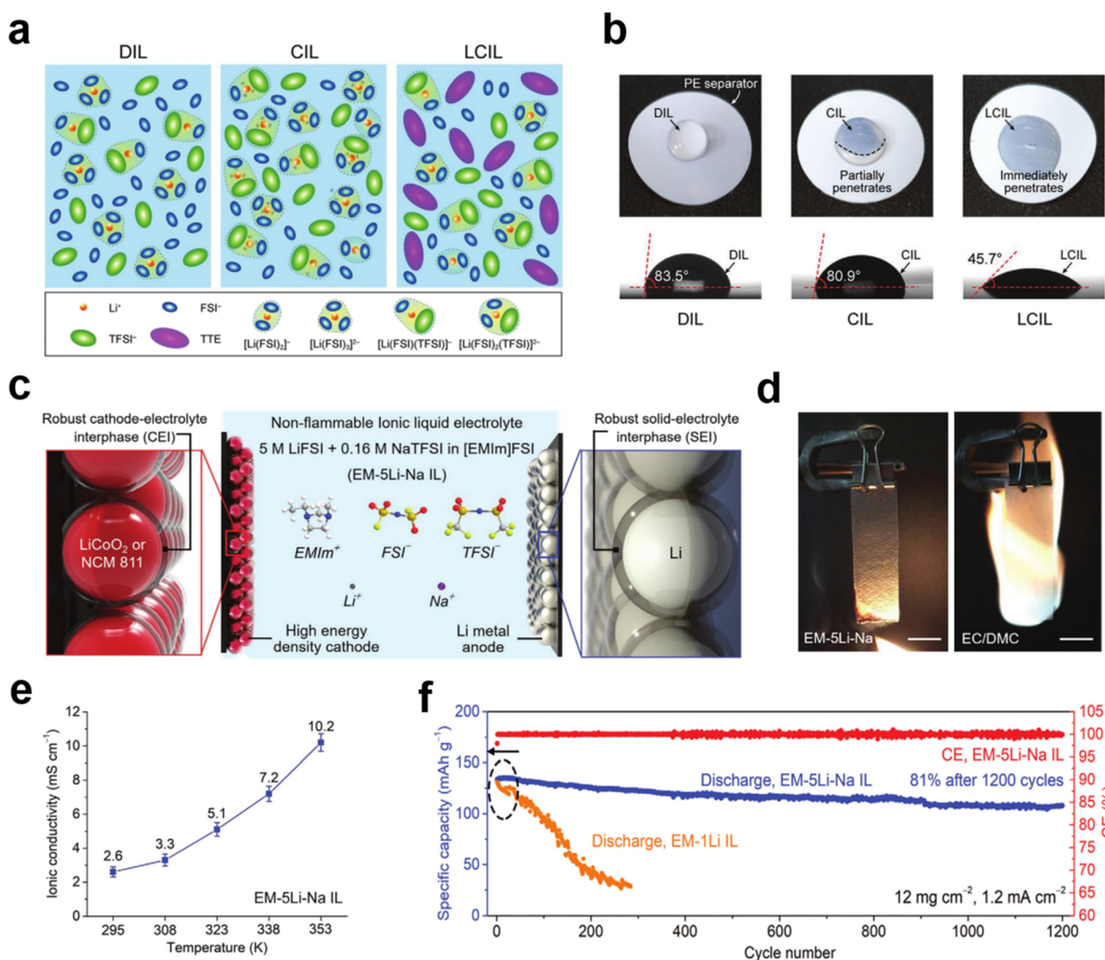
Fig. 2 (a) Schematic illustration of the solution structures of IL electrolytes; (b) photo images of wetting behavior and contact angles on PE separator. Reproduced with permission. 38 Copyright 2020, Wiley-VCH; (c) schematic illustration of the battery configuration and electrolyte composition of the EM-5Li-Na IL electrolyte; (d) flammability tests of the EM-5Li-Na IL electrolyte and conventional organic electrolyte consisting of 1 m LiPF 6 in EC/DMC (1:1 by vol); (e) ionic conductivity of the EM-5Li-Na IL at various temperatures; (f) cyclic stability of Li metal–LiCoO 2 batteries using EM-1Li and EM-5Li-Na IL electrolytes. Reproduced with permission. 42 Copyright 2020, Wiley-VCH.
