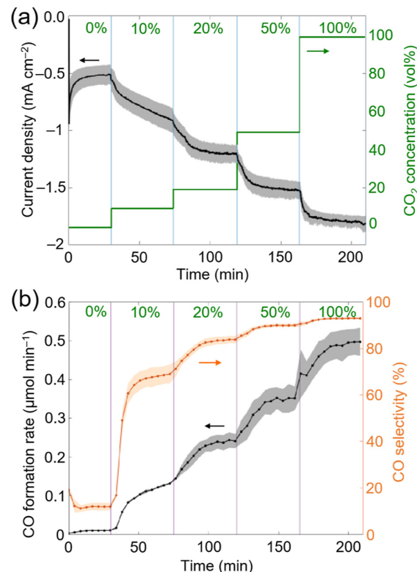
Fig. 3 (a) Chronoamperometry (CA) experiments as a function of concentration of \text{CO}_2 and time during \text{CO}_2 electrochemical reduction to \text{CO} using CP| CoP L cathodes. (b) \text{CO} formation rate and selectivity during CA experiments. Experiments were performed in triplicates, and the shaded area represents the standard deviation. Reaction conditions: CA: 0.1 M \text{NaHCO}_3 in \text{H}_2\text{O} (pH = 6.7); E_{\text{app}} = -1.2 \text{ V vs. Ag/AgCl} for 3.5 h; WE: CP| CoP L , CE: Pt foil, RE: Ag/AgCl (sat. KCl). Flow of \text{CO}_2 : \text{N}_2 9 \text{mL min}^{-1} . \text{CO}_2 concentration was varied stepwise between 0 vol%, 10 vol%, 20 vol%, 50 vol% and 100 vol% and balanced with \text{N}_2 .
