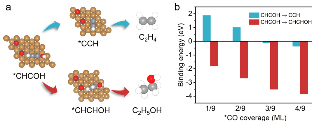
Fig. 4 DFT calculation results on the effects of *CO coverage. (a) Key reaction pathways for the CO_2RR to ethylene and ethanol on the Cu(111) surface. Yellow, copper; grey, carbon; red, oxygen; and white, hydrogen. (b) Binding energies of *CCH (cyan) and *CHCHOH (red) intermediates at different *CO coverages on the Cu(111) surface.
