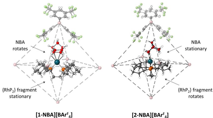
Fig. 10 Packing diagrams contrasting the relative orientations of the NBA and \{\text{RhP}_2\} fragments in [\text{1-NBA}][\text{BAR}^{\text{F}}_4] and [\text{2-NBA}][\text{BAR}^{\text{F}}_4] . The top anion is shown in full along with the B atoms of the other anions within the octahedral array. Carbon atoms of the \sigma -alkane ligands are highlighted in red.
