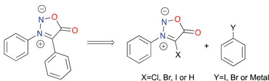
Scheme 1 Strategies for the mechanochemical \text{C}^4 -arylation of sydneses.
