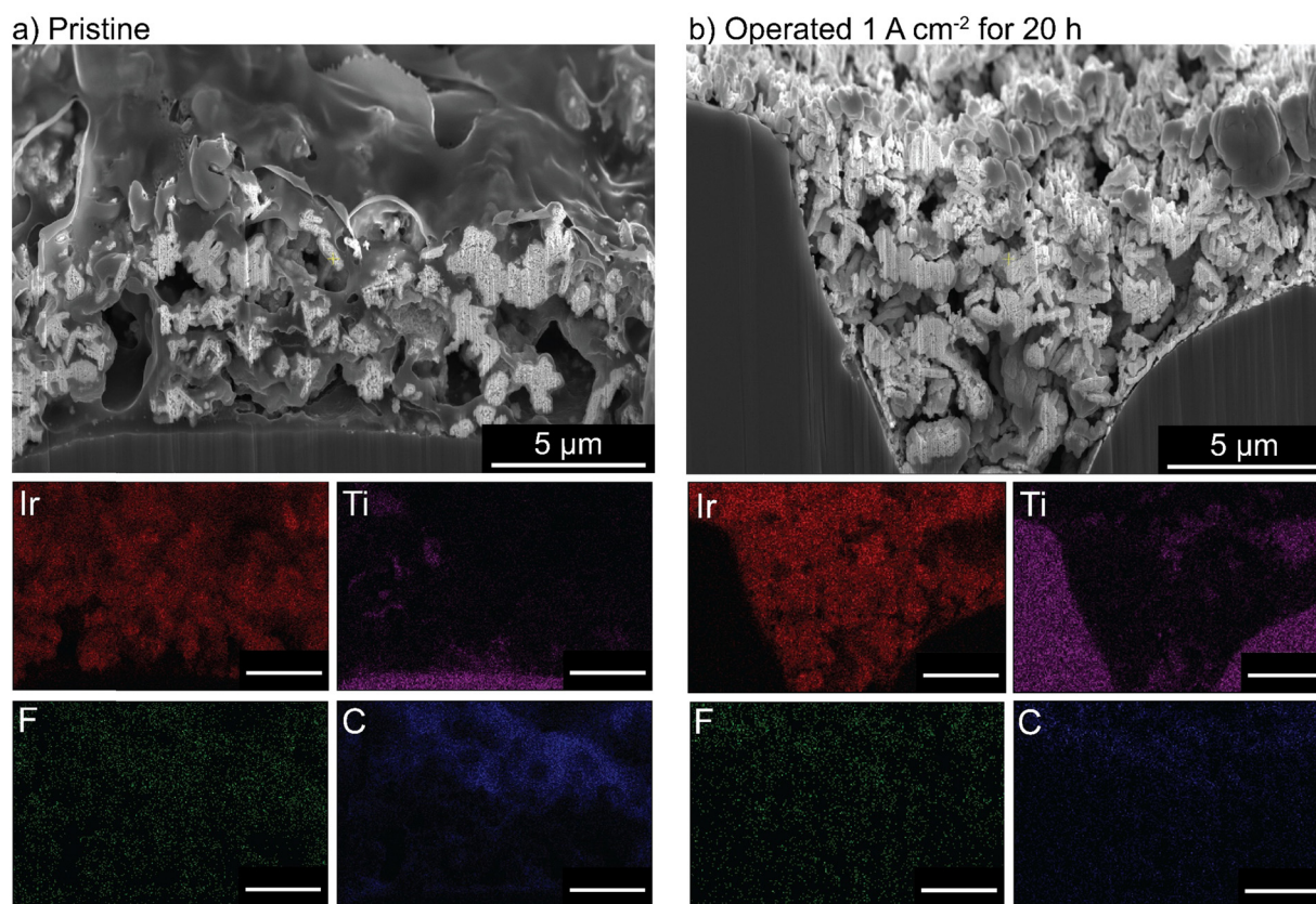
Fig. 5 Cross-sectional imaging and EDX of IrO x /20% TP-85 anode PTE. (a) Before and (b) after 20 h operation at 1 A cm -2 . All scale bars are 5 μm. No ionomer is observed in the catalyst layer after operation.
