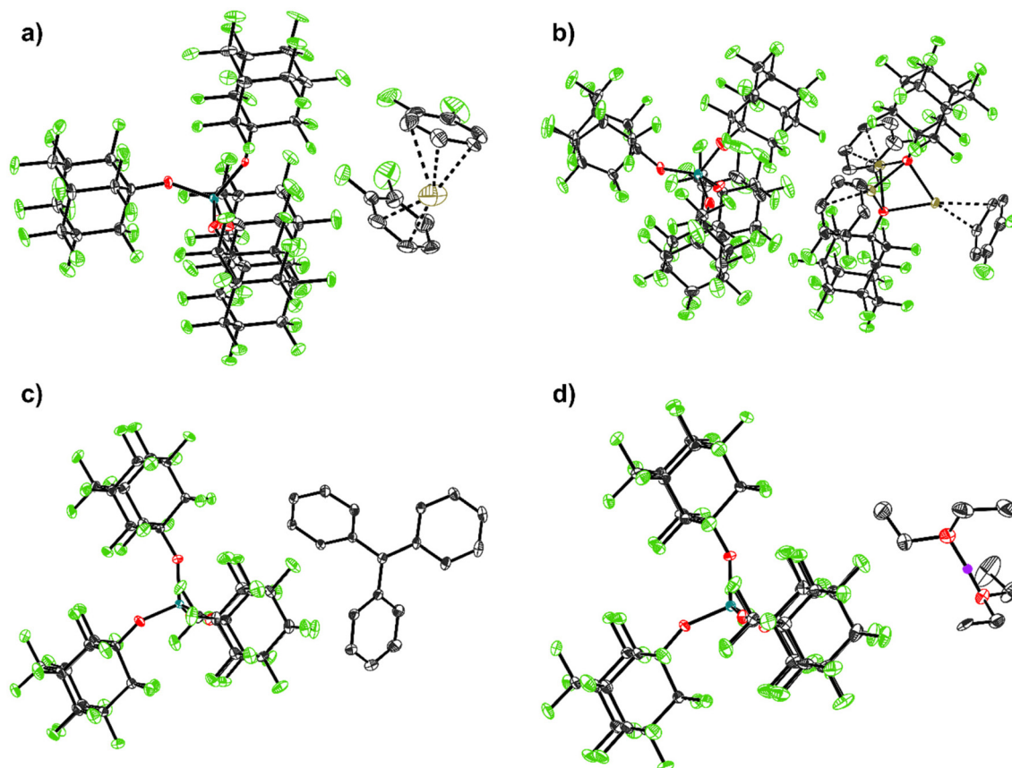
Fig. 2 Molecular structures of the structurally characterized [pfAd]^- salts: (a) [Ag(o\text{-DFB})_2][Al(OC_{10}F_{15})_4] (2- o -DFB), (b) [Ag_3(OC_{10}F_{15})_2(o\text{-DFB})_3][Al(OC_{10}F_{15})_4] (3), (c) [Ph_3C][Al(OC_{10}F_{15})_4] (4), (d) [H(OEt_2)_2][Al(OC_{10}F_{15})_4] (7). Hydrogen atoms are omitted for clarity with the exception for the acidic, bridging proton in (d) (purple). Disorders are omitted for clarity for (a) and (b) as well as two further o -DFB molecules with an occupation number of 4% in (b). The main occupation numbers are presented here. Thermal displacement ellipsoids were drawn at the 50% probability level. For details see ESI.†
