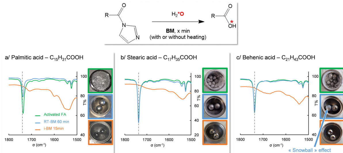
Fig. 5 Influence of i-BM on the isotopic labeling of fatty acids, as demonstrated using IR spectroscopy, for (a) palmitic acid ( T_{\text{melt}} \approx 73 \text{ }^\circ\text{C} ; T_{\text{i-BM}} = 70 \text{ }^\circ\text{C} ), (b) stearic acid ( T_{\text{melt}} \approx 78 \text{ }^\circ\text{C} ; T_{\text{i-BM}} = 85 \text{ }^\circ\text{C} ), and (c) behenic acid ( T_{\text{melt}} \approx 90 \text{ }^\circ\text{C} ; T_{\text{i-BM}} = 90 \text{ }^\circ\text{C} ). IR spectra of the activated FA (green), BM-hydrolysis test at room-temperature (blue, after 60 min milling) and under i-BM conditions (orange, after 15 min milling) are shown, with the dashed vertical line pointing to the C=O stretching frequency of the activated FA. Hydrolysis reactions were optimized using non-labeled or ^{18}\text{O} -enriched water (to check the feasibility of i-BM reactions), prior to working with ^{17}\text{O} -enriched water, in line with our previous work (which had shown that no isotopic effect on the hydrolysis rate would occur upon switching to ^{17}\text{O}/^{18}\text{O} -enriched water). Characterizations by mass-spectrometry of oxygen-labeled compounds are provided in ESI,† together with ^1\text{H} solution NMR analyses confirming the purity of the isolated products (Fig. S9–S13 in ESI†).
