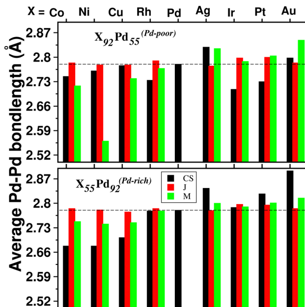
Fig. 4 Bar plot of average Pd–Pd nearest neighbor bond-lengths in the optimized Janus (J), core–shell (CS) and Mixed (M) structures for each bimetallic Pd 55 X 92 (top panel) and Pd 92 X 55 cluster (bottom panel). The corresponding value for the pristine Pd 147 cluster is indicated by the horizontal dashed line.
