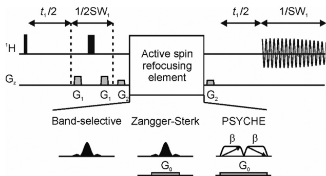
Fig. 2 Pulse sequences for pure shift NMR measurements using interferogram (pseudo-2D) acquisition. Narrow and wide rectangles represent hard 90° and 180° radiofrequency pulses, respectively. Various active spin refocusing (ASR) elements may be used, for example a selective 180° refocusing pulse with a simultaneous weak spatial encoding gradient G_0 (Zangger-Sterk) or without (band-selective), or a pair of low flip angle frequency swept pulses with a weak gradient (PSYCHE). Gradient pulses G_1 and G_2 enforce the required coherence transfer pathway (CTP). The incremented delays t_1/2 provide the evolution time required for interferogram acquisition.
