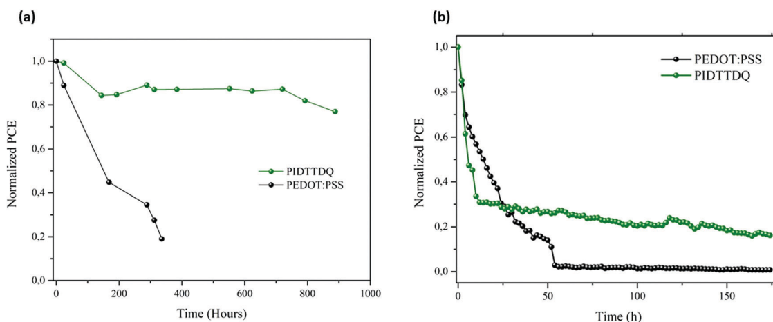
Fig. 7 (a) Device stability evaluation using the ISOS D1 Protocol. (b) Device lifetime investigation using the ISOS L2 protocol.
