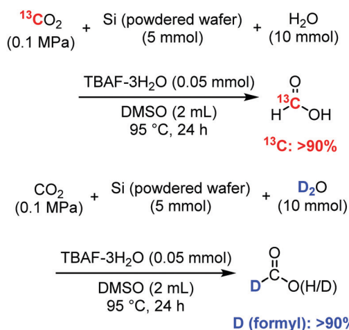
Scheme 1 Isotopic experiment. ^{13}\text{C} CO 2 : powdered silicon wafer (5 mmol; diameter < 20 μm), ^{13}\text{C} CO 2 (1 atm), H 2 O (10 mmol), TBAF-3H 2 O (0.05 mmol), DMSO (2 mL), 95 °C, 24 h. D 2 O: powdered silicon wafer (5 mmol; diameter < 20 μm), CO 2 (1 atm, balloon), D 2 O (10 mmol), TBAF-3H 2 O (0.05 mmol), DMSO (2 mL), 95 °C, 24 h.
