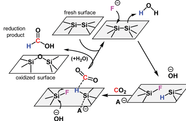
Scheme 2 Proposed catalytic reaction mechanism. A - : fluoride or hydroxide ion.
