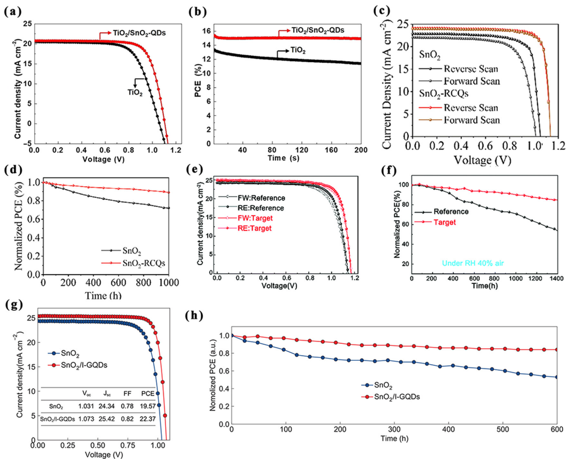
Fig. 7 QDs for the ETL/perovskite interfaces of normal structural PSCs. J - V curves (a) and stability curves (b) of PSCs based on pristine and \text{SnO}_2 -QDs. Reproduced with permission from ref. 73. Copyright 2019 Elsevier. J - V curves (c) and stability curves (d) of PSCs based on \text{SnO}_2 and \text{SnO}_2 -RCQs. Reproduced with permission from ref. 74. Copyright 2020 Wiley. J - V curves (e) and stability curves (f) of PSCs based on \text{SnO}_2 and \text{SnO}_2 /MQDs. Reproduced with permission from ref. 75. Copyright 2021 The Royal Society of Chemistry. J - V curves (g) and stability curves (h) of PSCs based on \text{SnO}_2 and \text{SnO}_2/\text{I-GQDs} . Reproduced with permission from ref. 76. Copyright 2021 Wiley.
