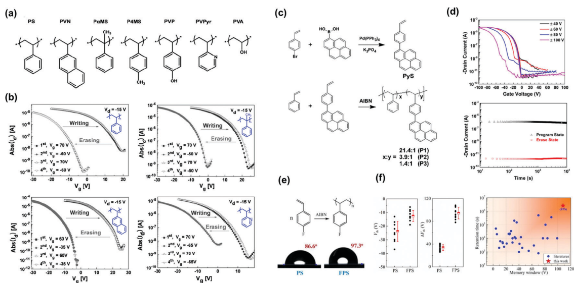
Fig. 3 Styrenic polymers as the charge trapping layer. (a) Chemical structure of styrenic polymer electrets; PS, PVN, PaMS, P4MS, PVP, PVPy, and PVA. (b) Reversible V_{th} shift in transfer plots of the OFET memory devices with various styrenic polymer gate electrets. Reproduced with permission. 29 Copyright 2008, Wiley-VCH. (c) Synthetic routes for P(St-co-Pys) polymers. (d) Transfer characteristics after electrical writing and erasing (top) and retention test (bottom) of the memory device comprising [P(St-co-Pys)] polymer electret. Reproduced with permission. 44 Copyright 2016, Wiley-VCH. (e) Chemical and physical characterization of FPS. (f) Statistics of V_{th} and V_{th} shift for PS and FPS (left) and Memory window and retention time of polymeric gate dielectrics applied in OFETs (right). Reproduced with permission. 45 Copyright 2020, The Royal Society of Chemistry.
