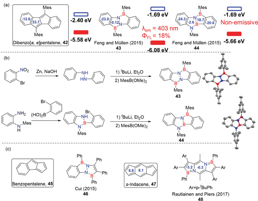
Fig. 14 (BN) 2 -Dibenzo[a,e]pentadienes. Crystal structures of 43 and 44 reprinted with permission from ref. 29. Copyright 2015 American Chemical Society.
