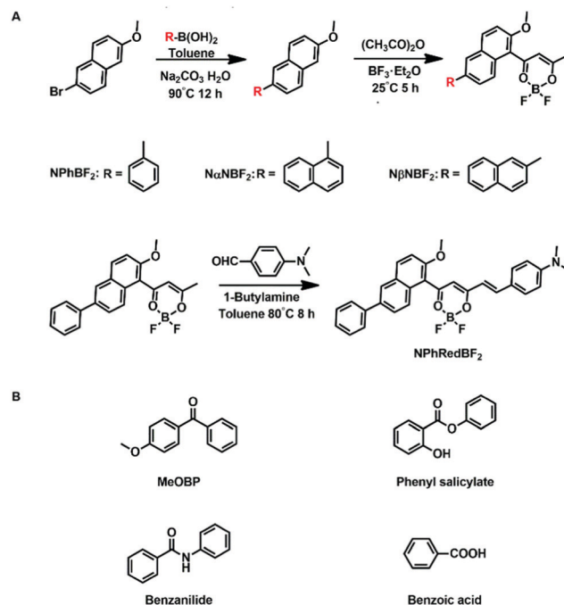
Scheme 2 Synthesis of naphthalene-containing \text{BF}_2\text{bdk} luminescent compounds via a cascade reaction and further modification.
