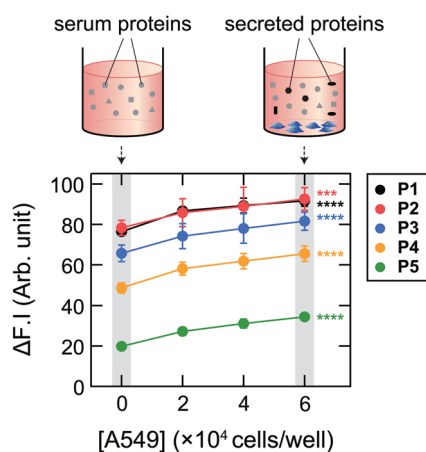
Fig. 3 Fluorescence responses of Dnc-polymers (2.0 μg mL -1 ) to 5.0 vol% spent media (collected after 48 h of incubation of A549 cells (seeded at 0–6.0 × 10 4 cells per well)) supplemented with 1.0 vol% FBS in 19 mM MOPS buffer (pH = 7.4); \lambda_{\text{ex}}/\lambda_{\text{em}} = 360 nm/480 nm. Mean values ± SD ( n = 6 ; two-tailed, unpaired, Student's t -test; *** P < 0.001 , **** P < 0.0001 ; 6 × 10 4 cells per well vs. no cells).
