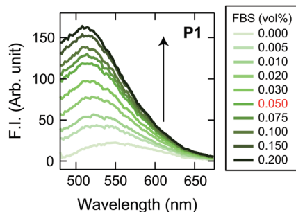
Fig. 2 Typical responses of a Dnc-polymer to FBS. Fluorescence spectra of P1 (2.0 μg mL -1 ) upon addition of FBS (0–0.2 vol%) in 19 mM MOPS buffer (pH = 7.4) with 5.0 vol% CDCHO; \lambda_{\text{ex}} = 360 nm. The volume fraction of FBS shown in red, i.e. , 5.0 vol% of spent CDCHO media supplemented with 1.0 vol% FBS, was chosen as the final concentration of spent medium to be added in the chemical-tongue analyses.
