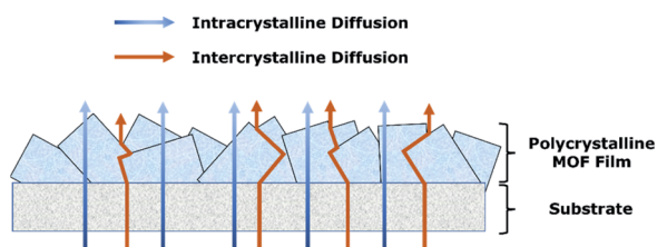
Fig. 6 Intracrystalline and intercrystalline transport through a polycrystalline MOF thin film.
