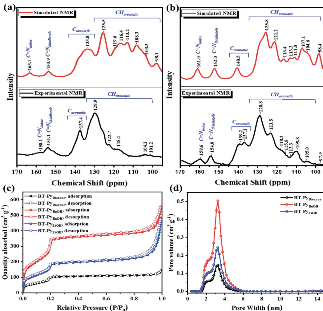
Fig. 2 Simulated and experimental ^{13}C -NMR spectra of the (a) BT-Py Solvent COFs and (b) BT-Cz Solvent COFs. (c) N 2 adsorption (solid symbols) and desorption (open symbols) isotherms of the BT-Py Solvent COFs at 77 K. (d) The pore-size distribution of the BT-Py Solvent COFs.
