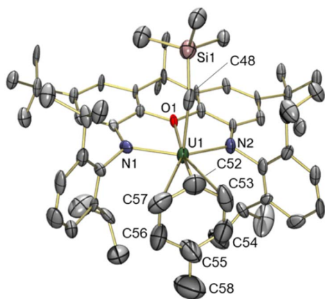
Fig. 4 X-ray crystal structure of [(\text{X}\text{A}_2)\text{U}(\text{CH}_2\text{SiMe}_3)(\eta^3\text{-C}_6\text{H}_5\text{Me})][\text{B}(\text{C}_6\text{F}_5)_4]\cdot\text{toluene} ( 3-toluene ), with thermal ellipsoids at 50% probability. Hydrogen atoms, the borate anion and a non-coordinated toluene solvent molecule are omitted for clarity. Selected bond distances (Å) and angles ( ^\circ ): U(1)–O(1) 2.417(9), U(1)–N(1) 2.22(1), U(1)–N(2) 2.21(1), U(1)–C(48) 2.36(2), U(1)–C(52) 3.05(2), U(1)–C(53) 3.13(2), U(1)–C(54) 3.47(2), U(1)–C(55) 3.78(2), U(1)–C(56) 3.70(2), U(1)–C(57) 3.36(2), U(1)–C arene ave. 3.42, U(1)–Centroid 3.14, C(55)–C(58) 1.46(3), U(1)–C(48)–Si(1) 136.8(7), O(1)–U(1)–C(48) 88.8(4), N(1)–U(1)–N(2) 128.0(4).
