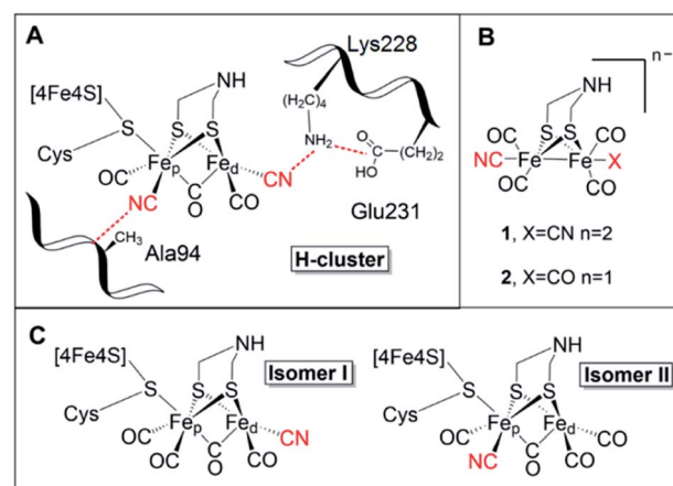
Fig. 1 (A) Schematic representation of the active site of [FeFe] hydrogenase, the H-cluster, and selected amino acids (numbering based on CrHydA1). (B) The synthetic mimics used in this study [\text{Fe}_2(\mu\text{-adt})(\text{CO})_4(\text{CN})_2]^{2-} (1) and [\text{Fe}_2(\mu\text{-adt})(\text{CO})_5(\text{CN})]^- (2). (C) Possible H-cluster isomer forms following maturation of apo-hydrogenase using complex 2. Cyanide ligands are highlighted in red. Possible rotamers of isomer II are shown in Fig. S9.†
