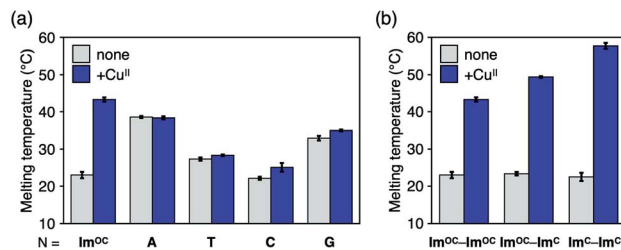
Fig. 5 (a) Melting temperatures of duplexes containing an \text{Im}^{\text{OC}}\text{-N} base pair ( 1 \cdot 2\text{N} ; N = \text{A}, \text{T}, \text{C}, \text{G} ) in the absence and presence of 1 equiv. of \text{Cu}^{\text{II}} . (b) Melting temperatures of duplexes containing an \text{Im}^{\text{OC}}\text{-Im}^{\text{OC}} ( 1 \cdot 2 ), an \text{Im}^{\text{OC}}\text{-Im}^{\text{C}} ( 1 \cdot 8 ), or an \text{Im}^{\text{C}}\text{-Im}^{\text{C}} base pair ( 7 \cdot 8 ) in the absence and presence of 1 equiv. of \text{Cu}^{\text{II}} . [duplex] = 2.0 μM and [\text{Cu}^{\text{II}}]/[\text{duplex}] = 0 or 1 in 10 mM HEPES buffer (pH 7.0) and 100 mM NaCl. N = 3 . The error bars represent the standard errors.
