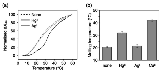
Fig. 4 (a) Melting curves of a DNA duplex containing an \text{Im}^{\text{OC}}\text{-Im}^{\text{OC}} base pair ( 1 \cdot 2 ) in the presence of Hg II and Ag I ions. [duplex] = 2.0 μM, [metal ion]/[duplex] = 0 (dashed line) or 1 (solid lines) in 10 mM HEPES buffer (pH 7.0), 100 mM NaNO 3 , 0.2 °C min -1 . (b) Melting temperatures. N = 3 . The error bars represent the standard errors. The melting temperature in the same buffer in the presence of Cu II is also shown.
